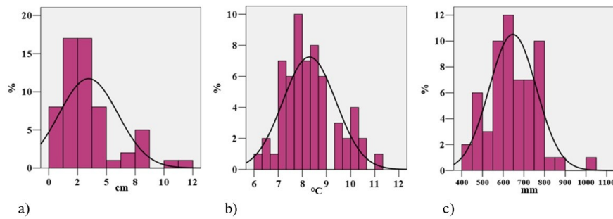
Figure 1 - Histogram of frequency distribution of climatic characteristics for 1961-2020: a – average ten-day snow depth; b – temperature; c – amount of precipitation
