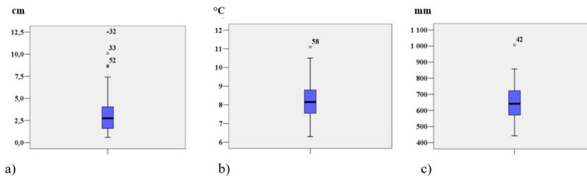
Figure 2 - Box plot with median and extremes for 1961-2020: a – average ten-day snow depth; b – temperature; c – amount of precipitation
